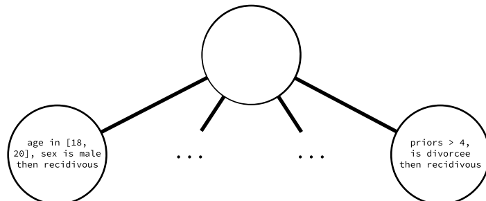
A branch and bound tree for rule lists, trimmed at depth 1.
